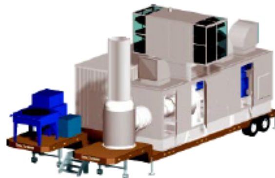
Sited Configuration of Taurus 60 Mobile Power Unit
