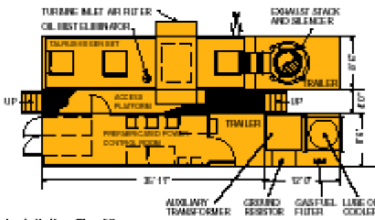
Installation Plan View
